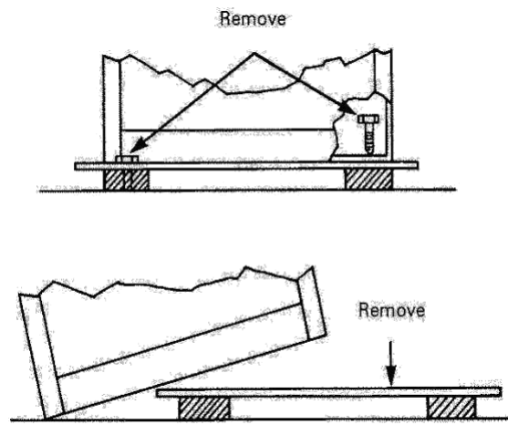
Figure 2: Removing the Shipping Bolts and Sliding the Unit Off the Skid
